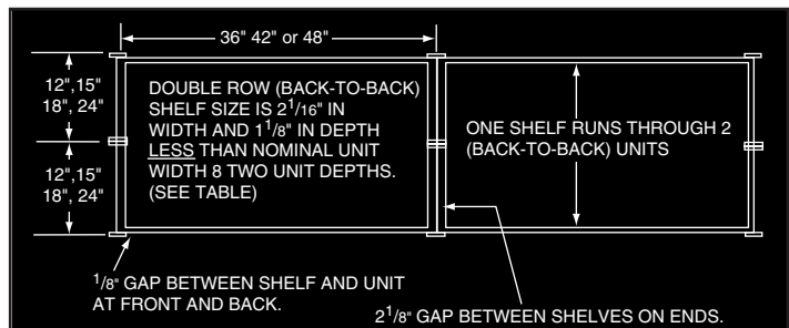
Typical Plan View – Double Row Units, Back to Back with Plywood Shelves.
